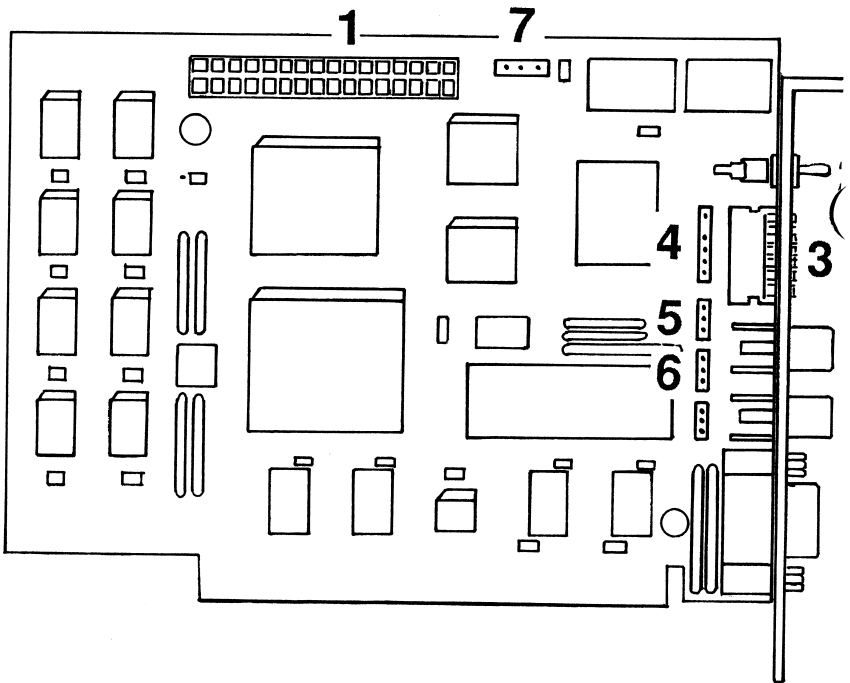
FIGURE 2. VEGA DELUXE CONNECTORS AND SWITCHES
